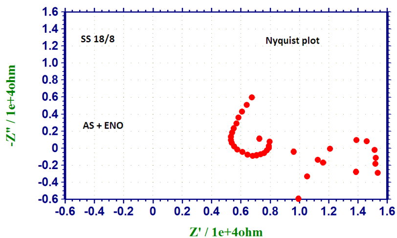
Figure 4. AC impedance spectrum of SS 18/8 immersed in Artificial Saliva+ENO (Nyquist plot).
