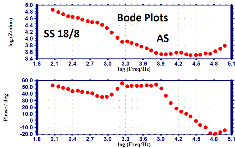
Figure 6. AC impedance spectrum of SS 18/8 immersed in Artificial Saliva (Bode plots).
