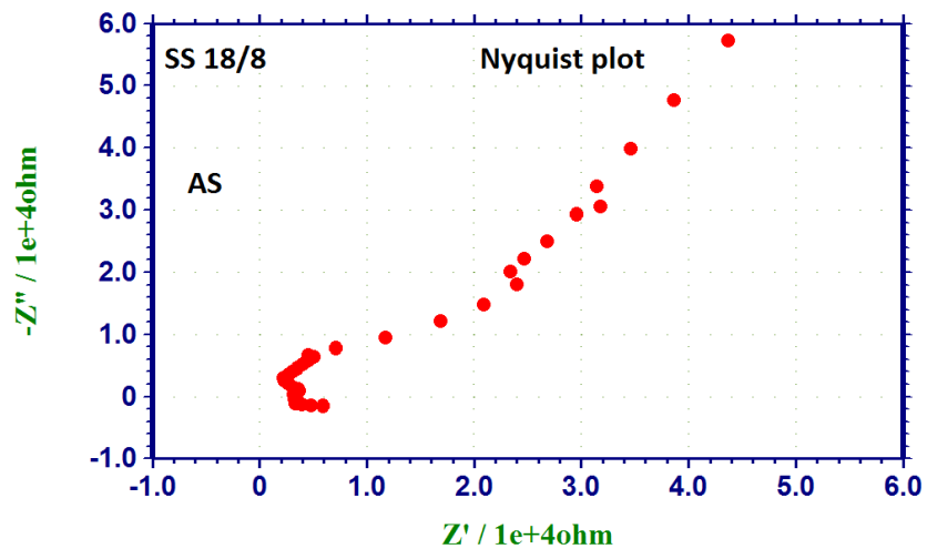
Figure 3. AC impedance spectrum of SS 18/8 immersed in Artificial Saliva (Nyquist plot).
