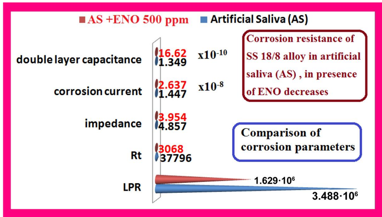
Figure 8. Corrosion resistance of SS 18/8 alloy in artificial saliva (AS) in the presence of ENO decreases.
