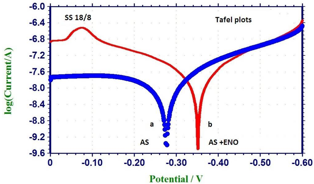
Figure 1. Polarisation curves of SS 18/8 alloy immersed in various test solutions.
