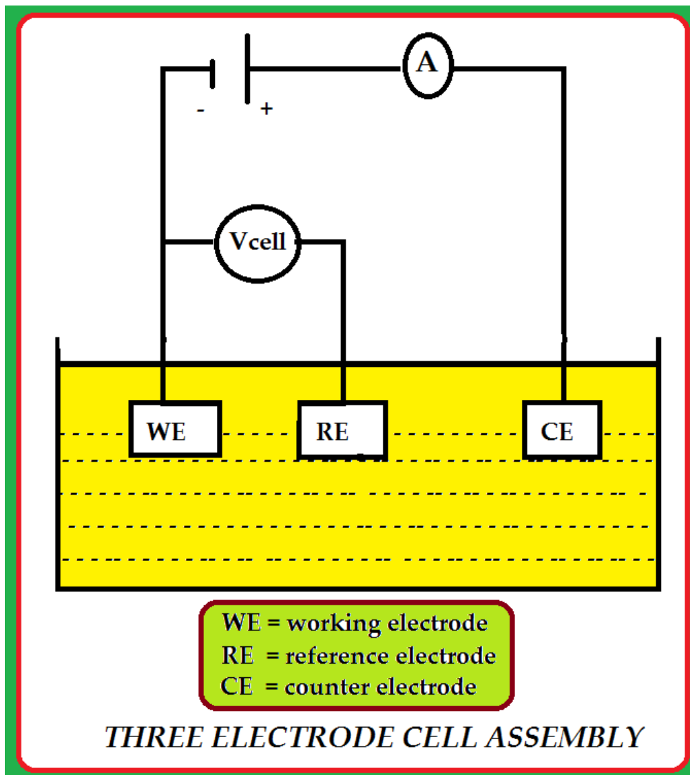
Scheme A. Three electrode cell assembly.
