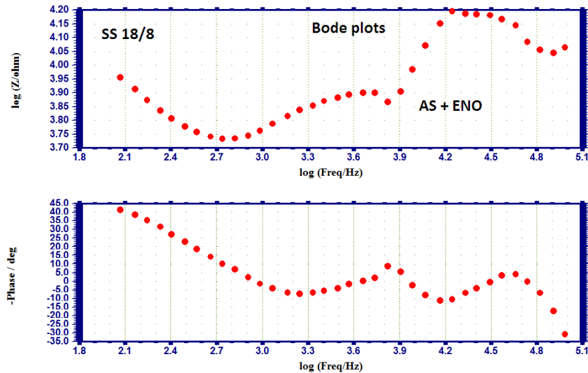
Figure 7. AC impedance spectrum of SS 18/8 immersed in Artificial Saliva+ENO (Bode plots).
